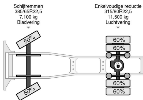
Volvo FH 440 GLOBETROTTER-XL (I-SHIFT / ENGINE... 4x2
