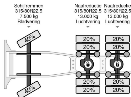
MAN 26.403 DFS 6x4 TRACTOR UNIT (EURO 2 / MANUAL ...
