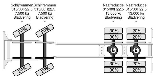
Scania R124-420 C 8x4 FULL STEEL CHASSIS (EURO 3 / F...
