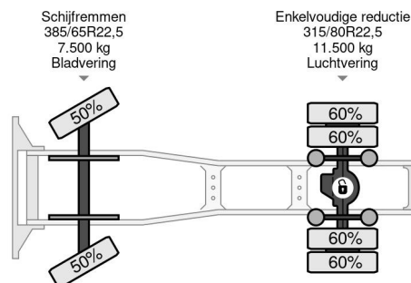
Scania R500 V8 TOPLINE (SEMI AUTOMATIC WITH C... 4x2
